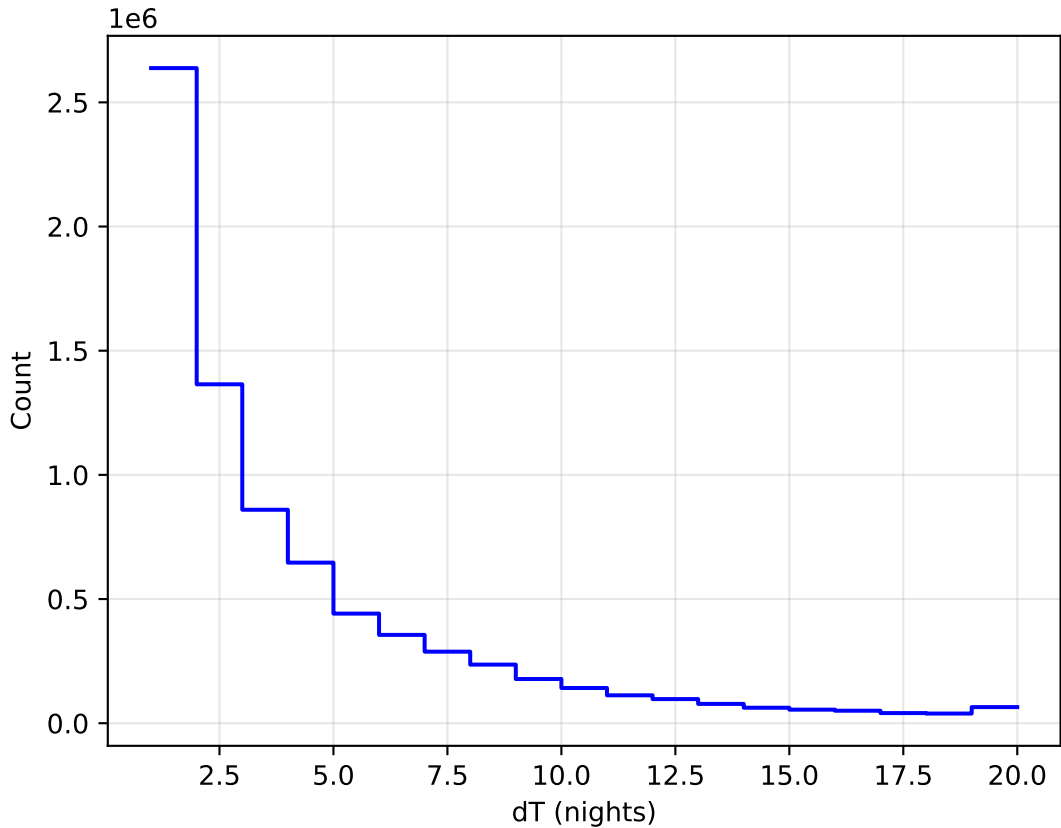
reweight_plane_v3.3_10yrs WFD all bands: DeltaNight Histogram
