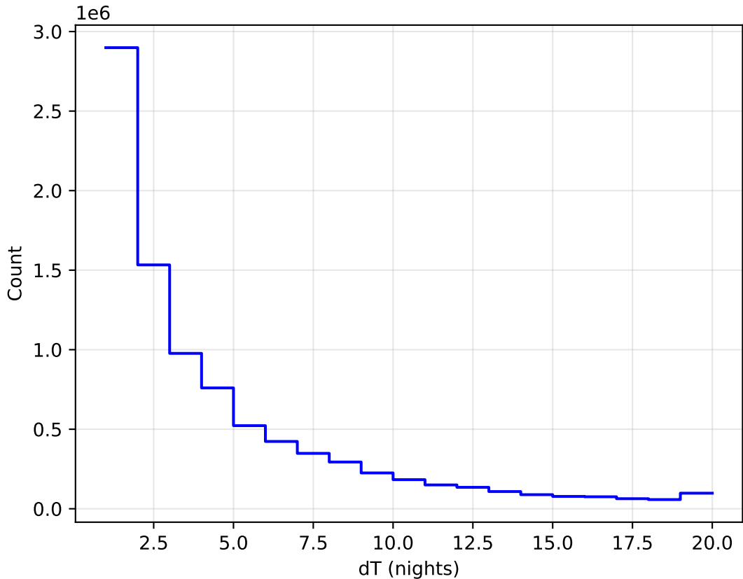
reweight_plane_v3.3_10yrs All sky all bands: DeltaNight Histogram
