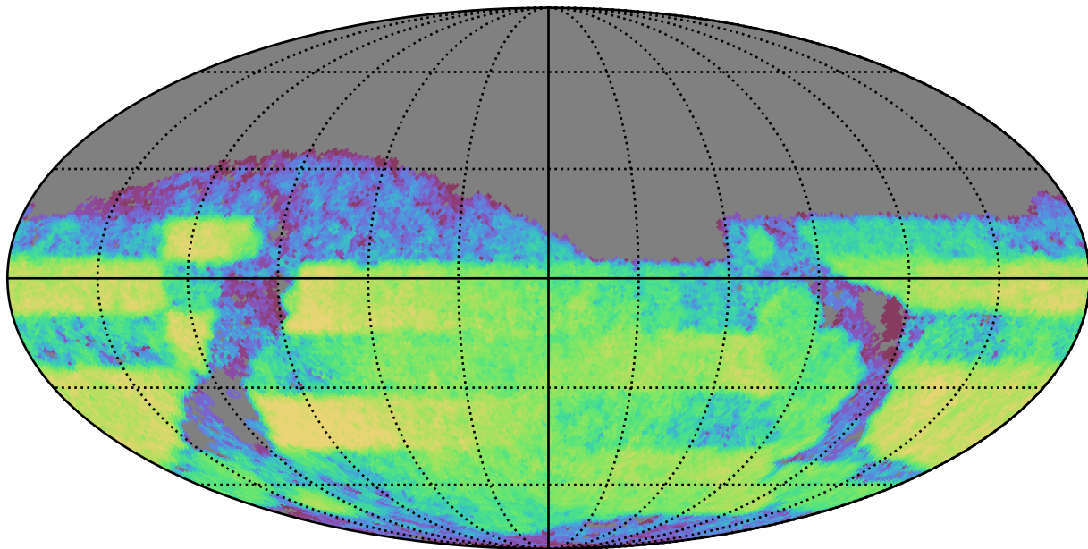
reweight_plane_v3.3_10yrs Yr 3-4 z band: CoaddM5
