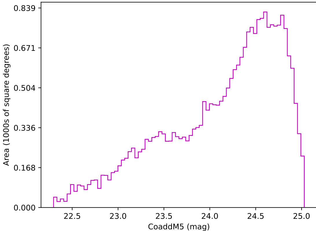
reweight_plane_v3.3_10yrs Yr 3-4 z band: CoaddM5
