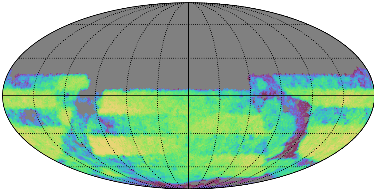
reweight_plane_v3.3_10yrs Yr 3-4 y band: CoaddM5
