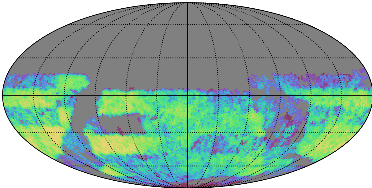
reweight_plane_v3.3_10yrs Yr 3-4 u band: CoaddM5
