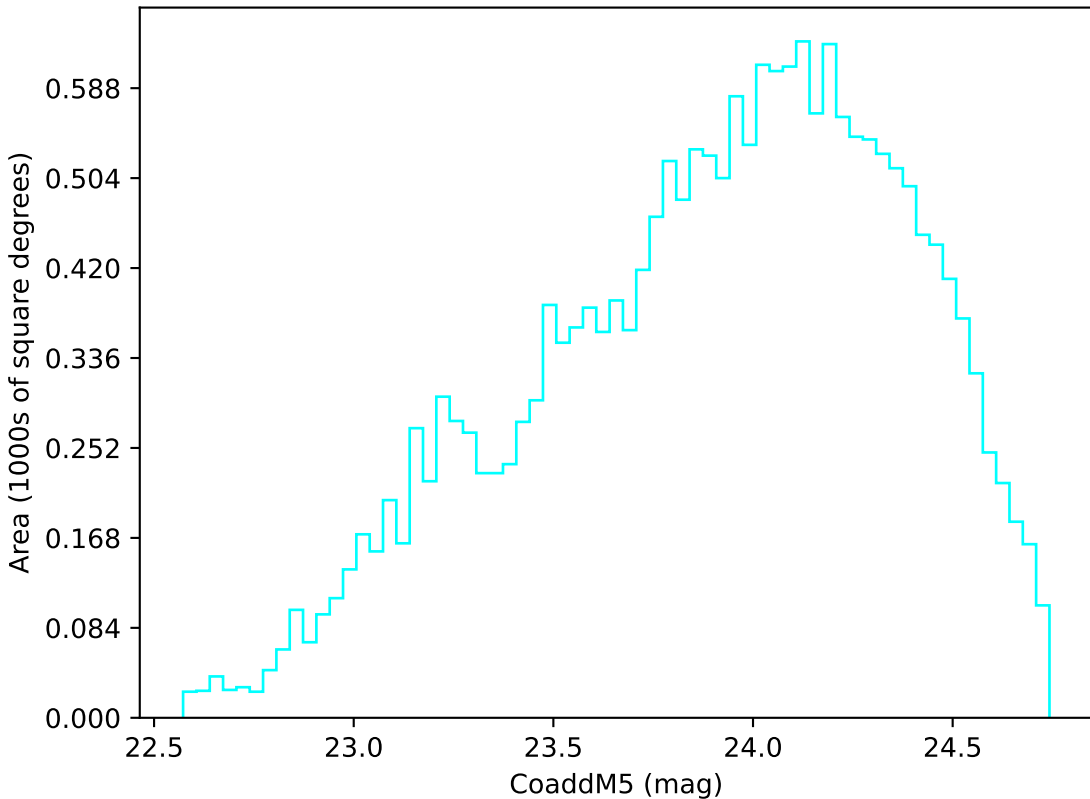
reweight_plane_v3.3_10yrs Yr 3-4 u band: CoaddM5
