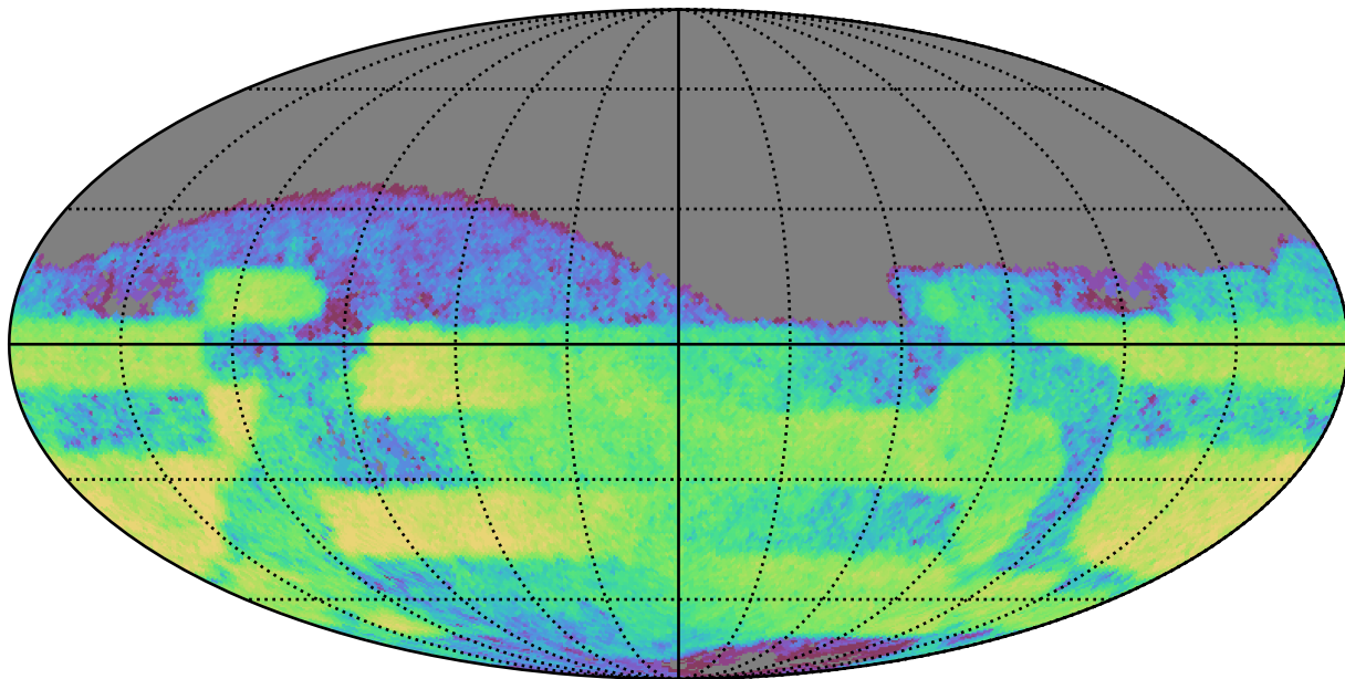
reweight_plane_v3.3_10yrs Yr 3-4 r band: CoaddM5
