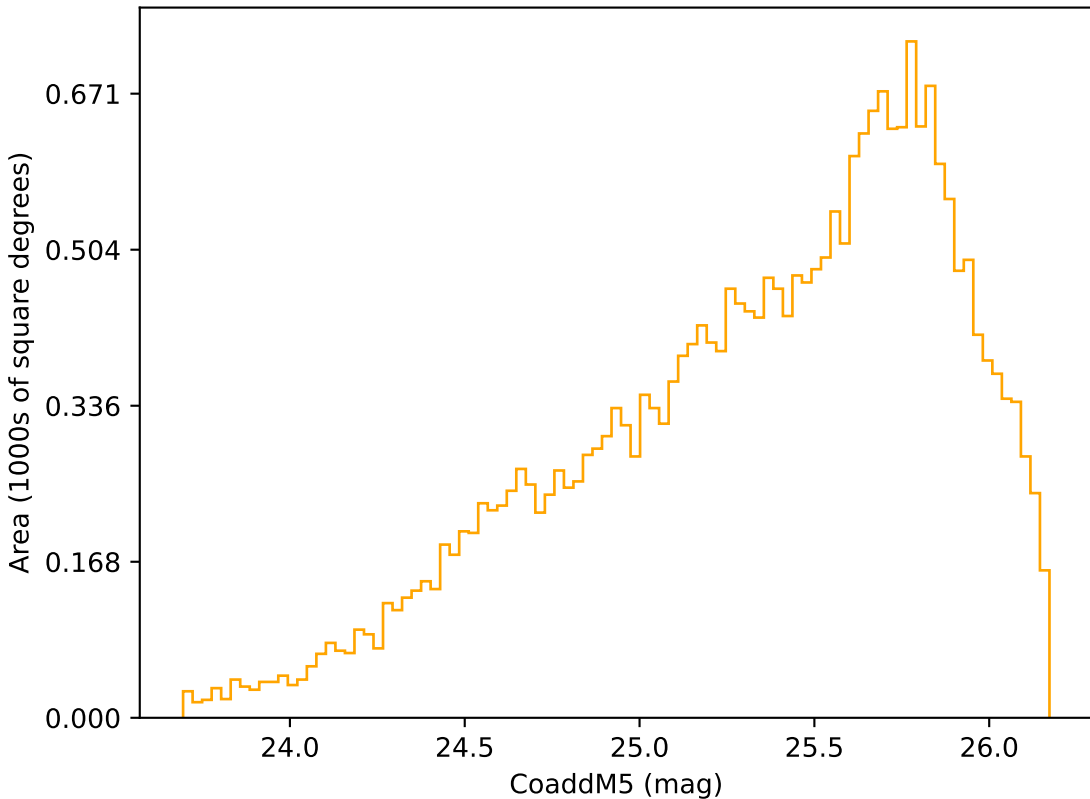
reweight_plane_v3.3_10yrs Yr 3-4 r band: CoaddM5
