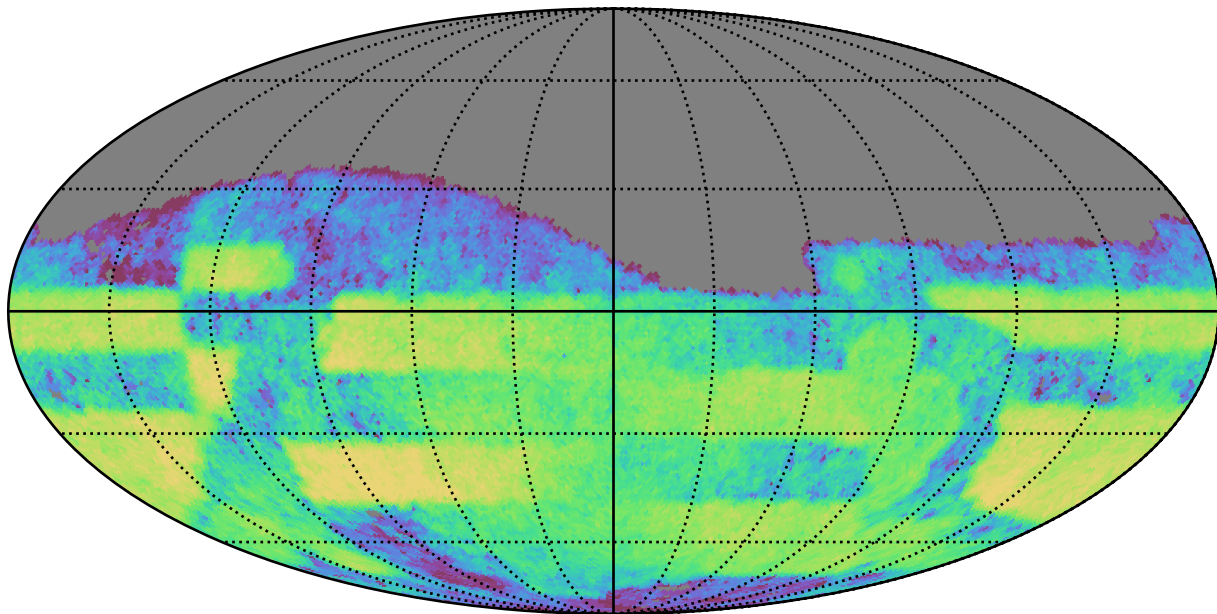
reweight_plane_v3.3_10yrs Yr 3-4 i band: CoaddM5
