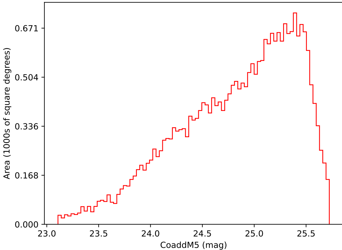
reweight_plane_v3.3_10yrs Yr 3-4 i band: CoaddM5
