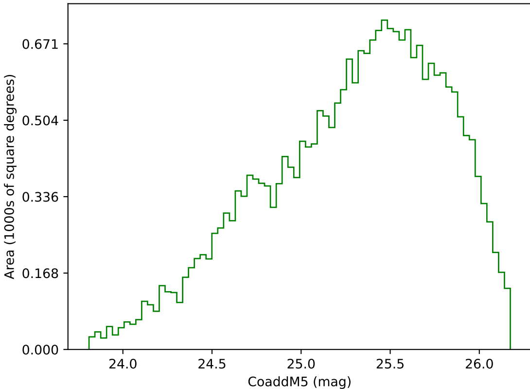
reweight_plane_v3.3_10yrs Yr 3-4 g band: CoaddM5
