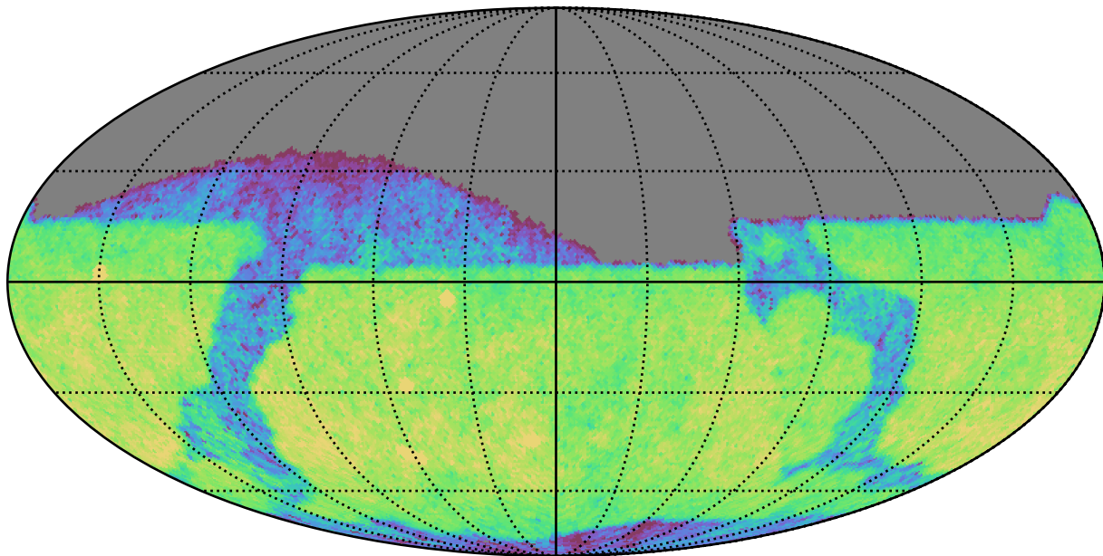
reweight_plane_v3.3_10yrs Yr 1 z band: CoaddM5
