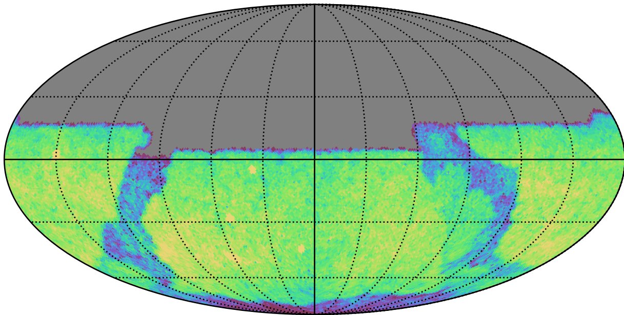
reweight_plane_v3.3_10yrs Yr 1 y band: CoaddM5
