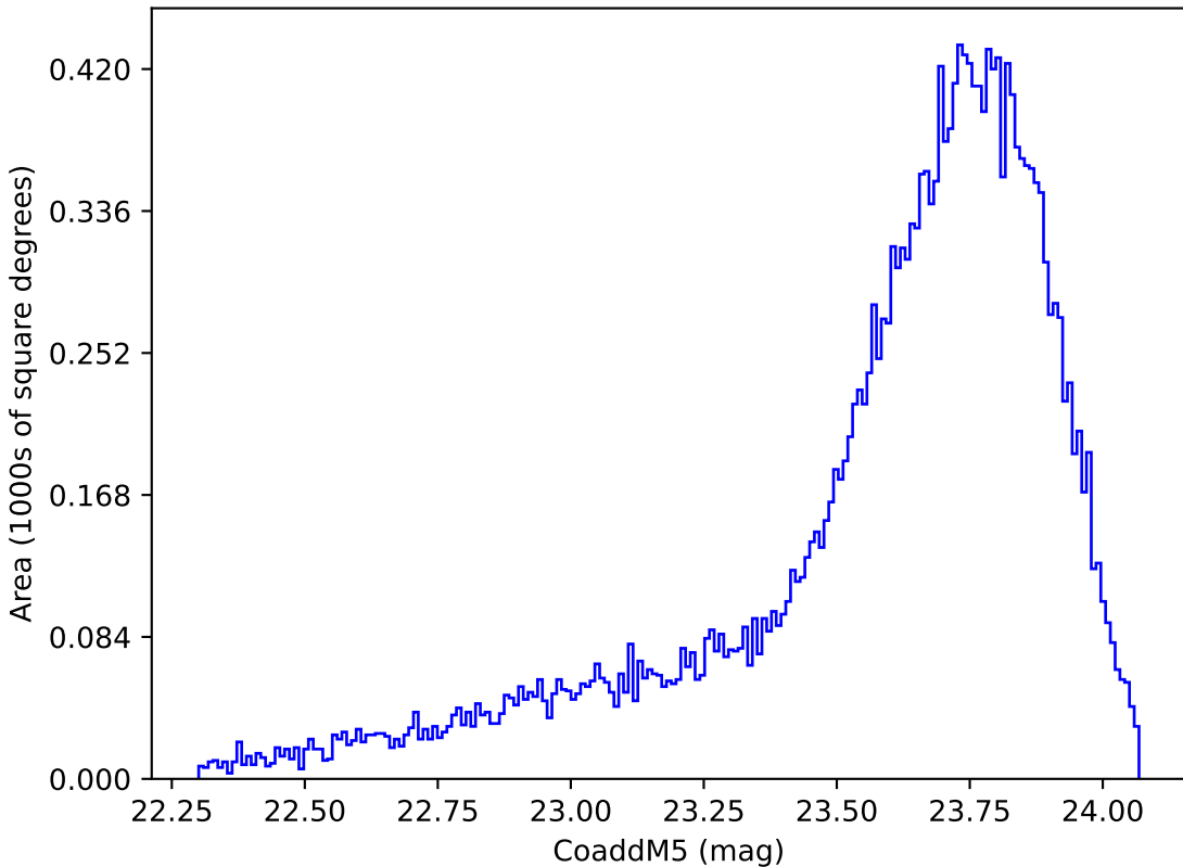
reweight_plane_v3.3_10yrs Yr 1 y band: CoaddM5
