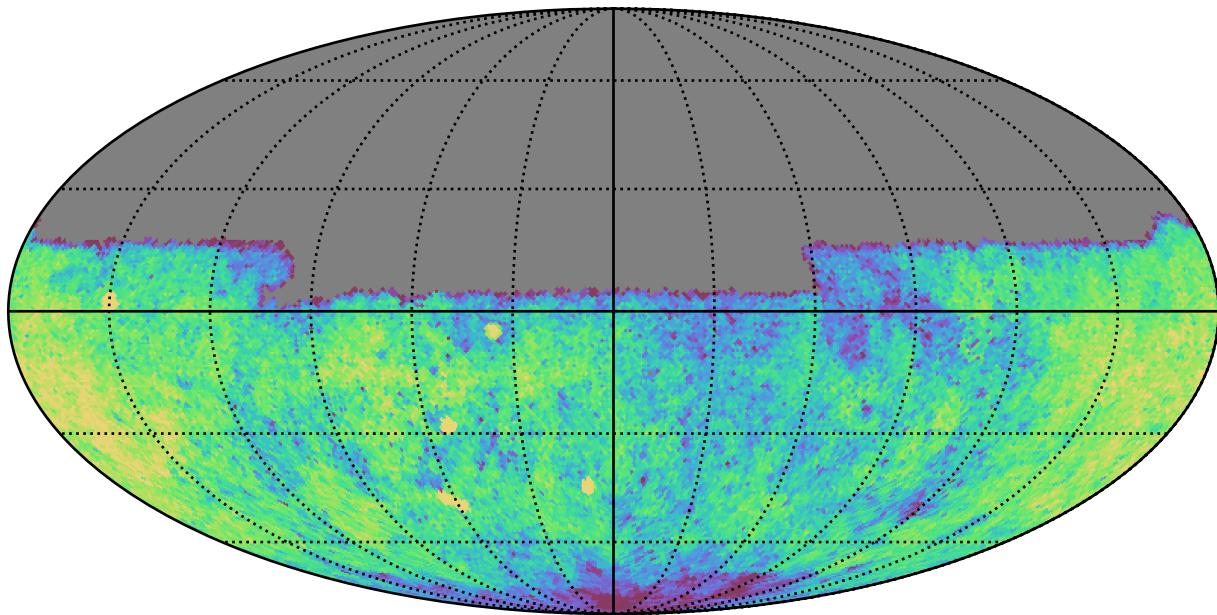
reweight_plane_v3.3_10yrs Yr 1 u band: CoaddM5
