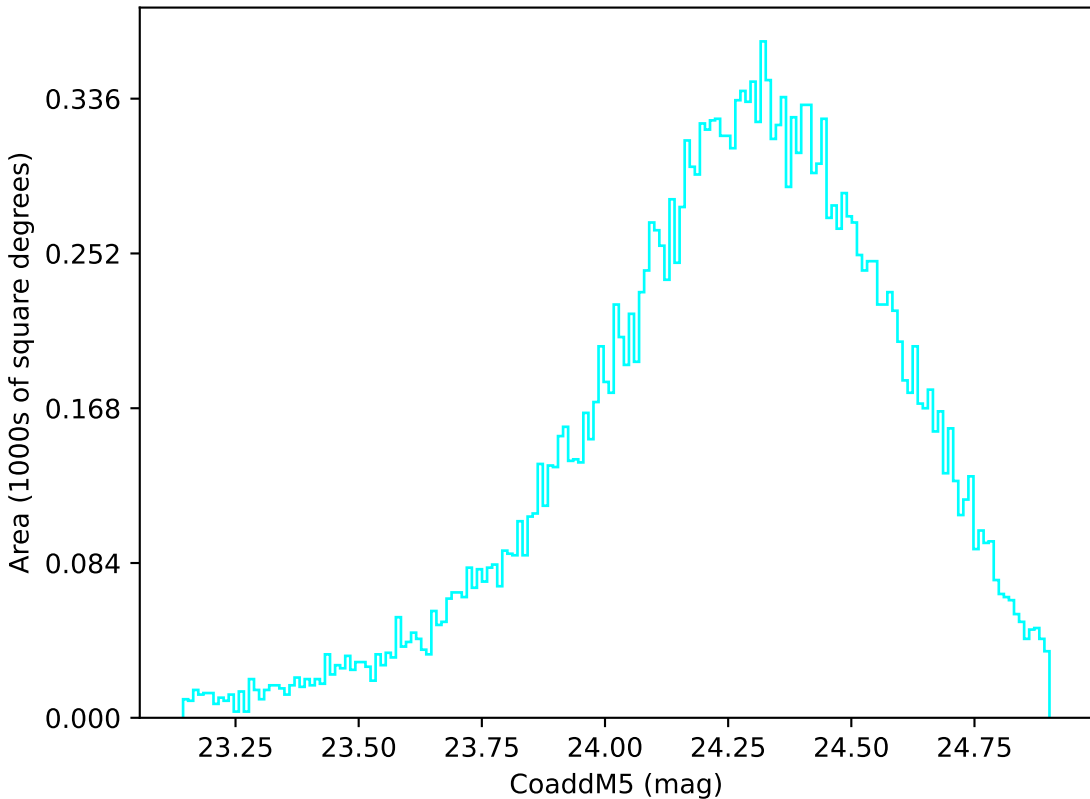
reweight_plane_v3.3_10yrs Yr 1 u band: CoaddM5
