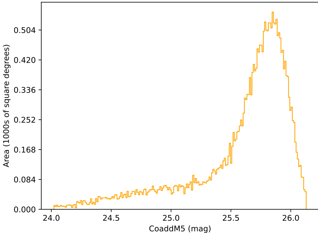
reweight_plane_v3.3_10yrs Yr 1 r band: CoaddM5
