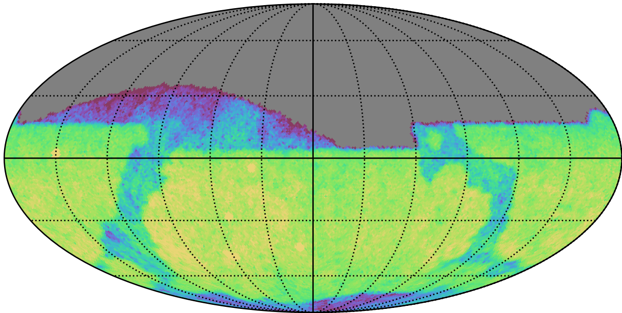
reweight_plane_v3.3_10yrs Yr 1 i band: CoaddM5
