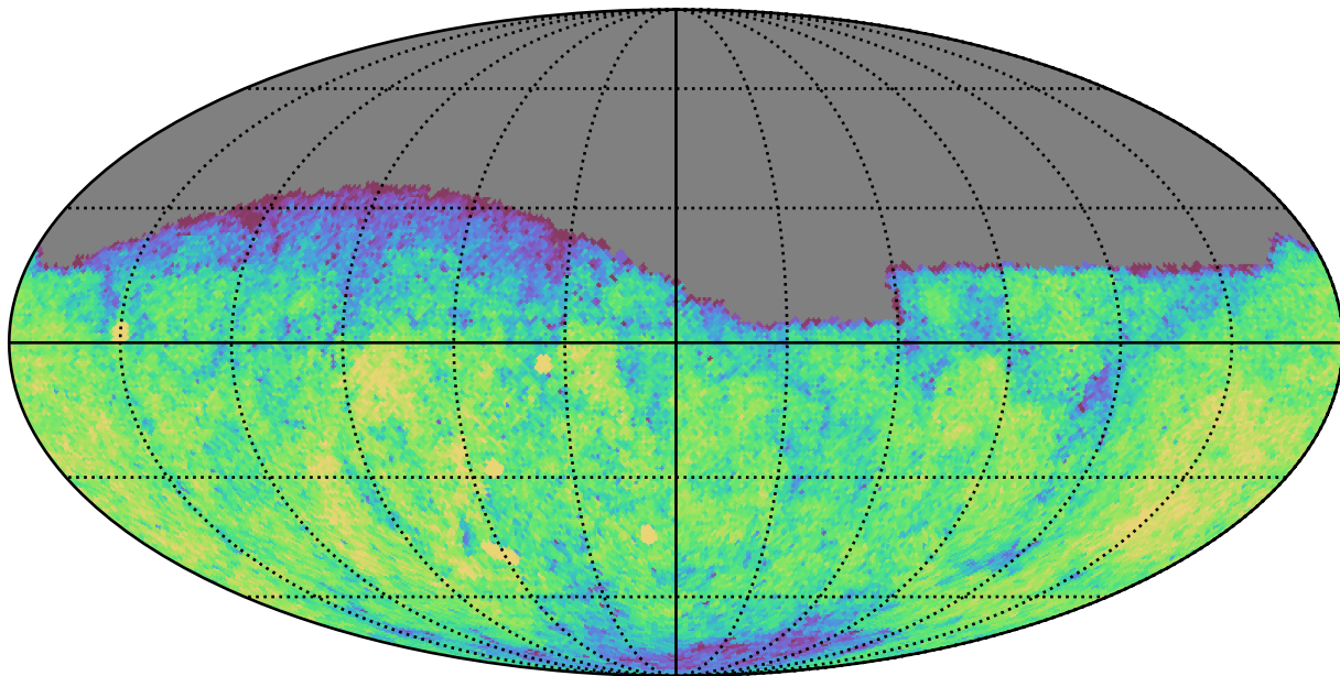
reweight_plane_v3.3_10yrs Yr 1 g band: CoaddM5
