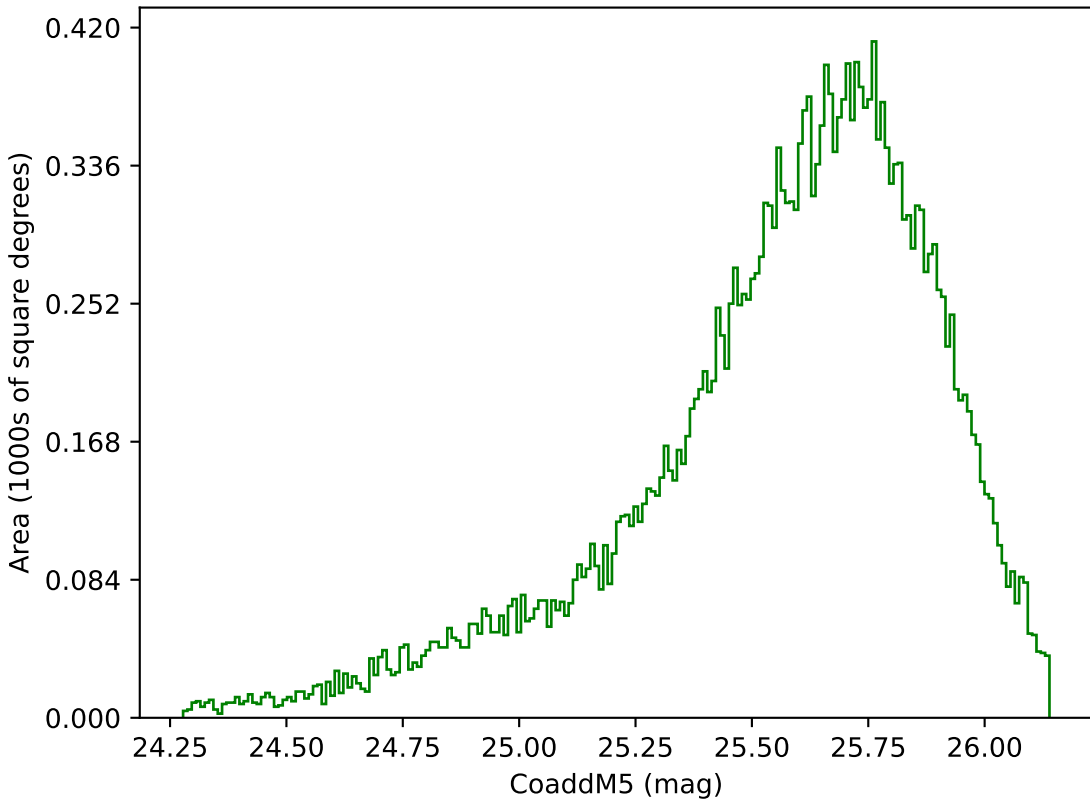
reweight_plane_v3.3_10yrs Yr 1 g band: CoaddM5
