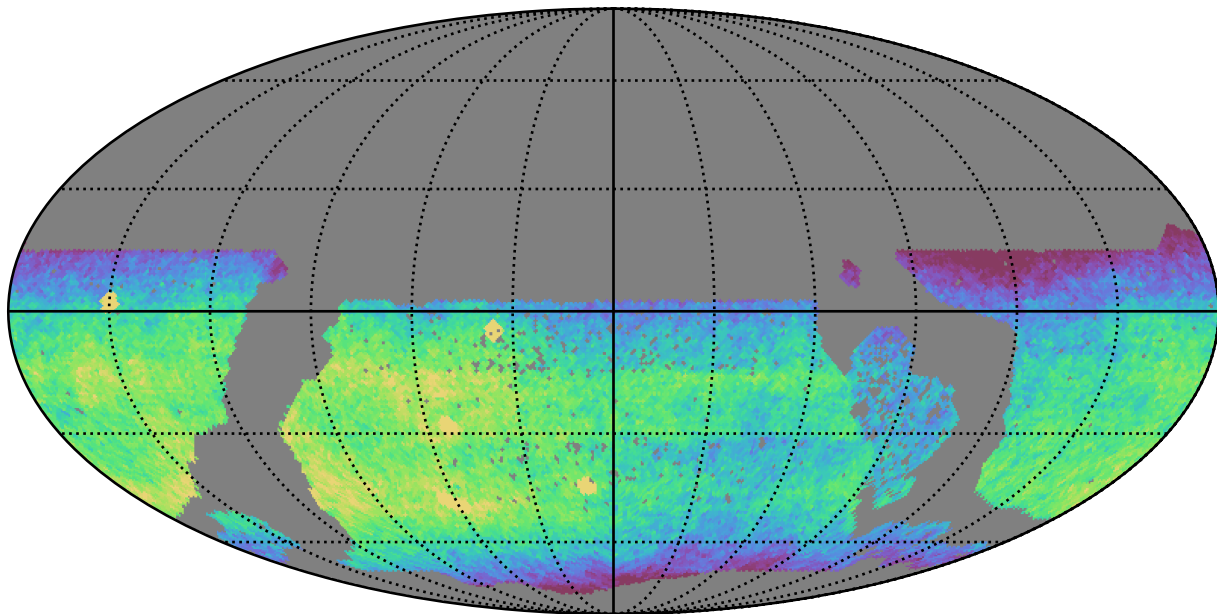
reweight_plane_v3.3_10yrs WFD z band: CoaddM5
