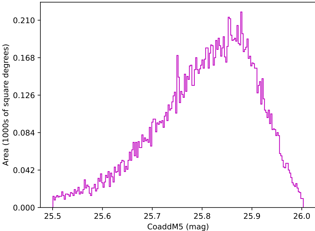
reweight_plane_v3.3_10yrs WFD z band: CoaddM5
