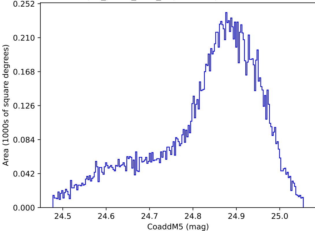
reweight_plane_v3.3_10yrs WFD y band: CoaddM5
