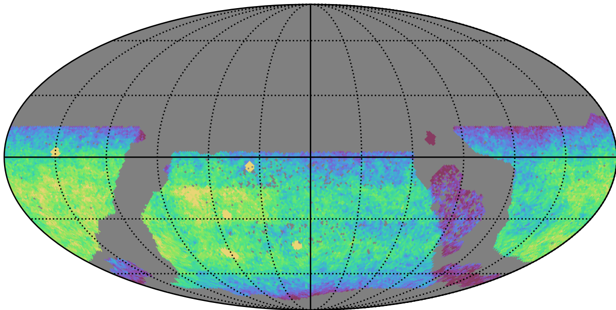
reweight_plane_v3.3_10yrs WFD u band: CoaddM5
