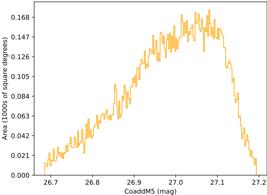
reweight_plane_v3.3_10yrs WFD r band: CoaddM5
