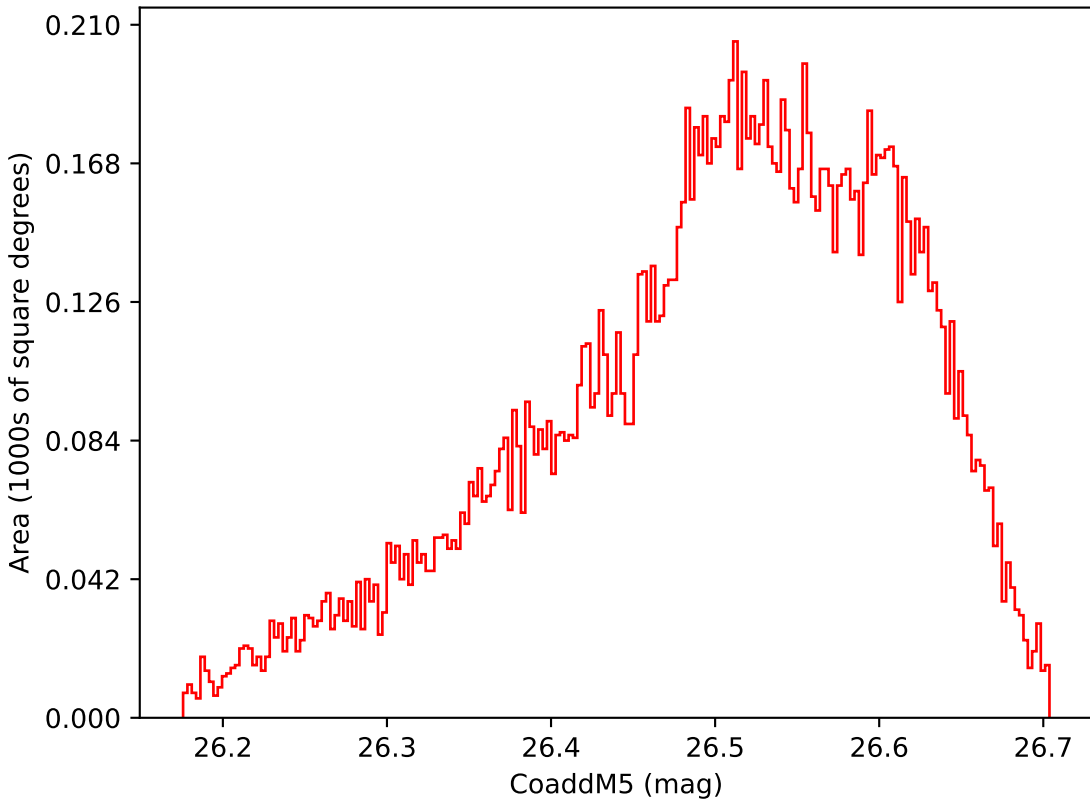
reweight_plane_v3.3_10yrs WFD i band: CoaddM5
