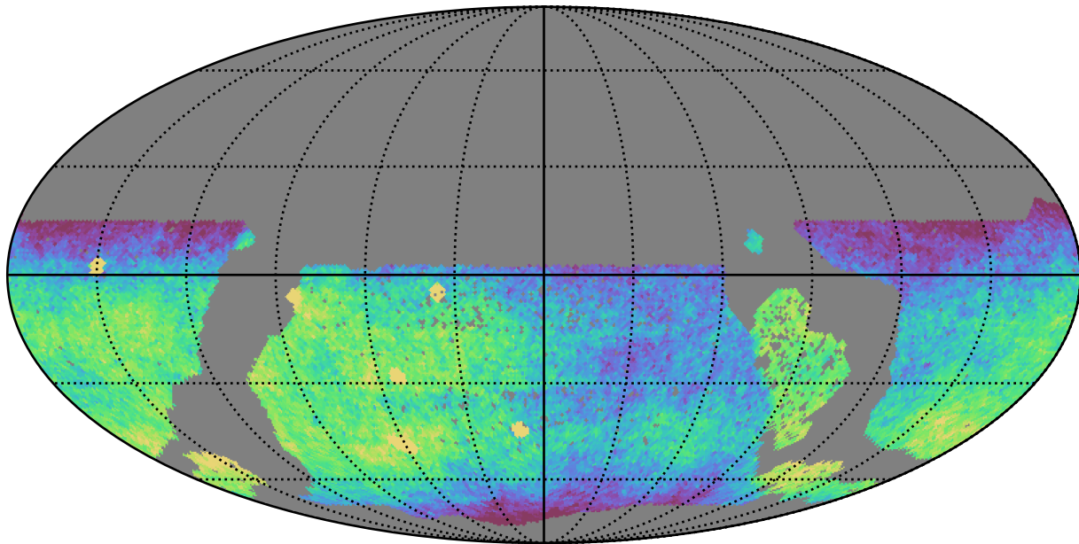
reweight_plane_v3.3_10yrs WFD g band: CoaddM5
