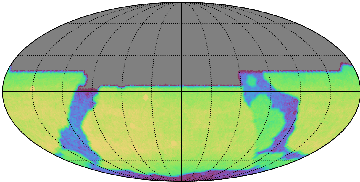
reweight_plane_v3.3_10yrs All sky y band: CoaddM5
