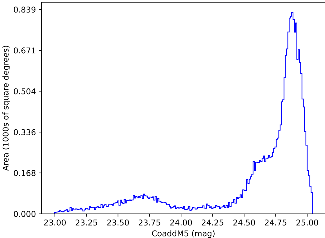
reweight_plane_v3.3_10yrs All sky y band: CoaddM5
