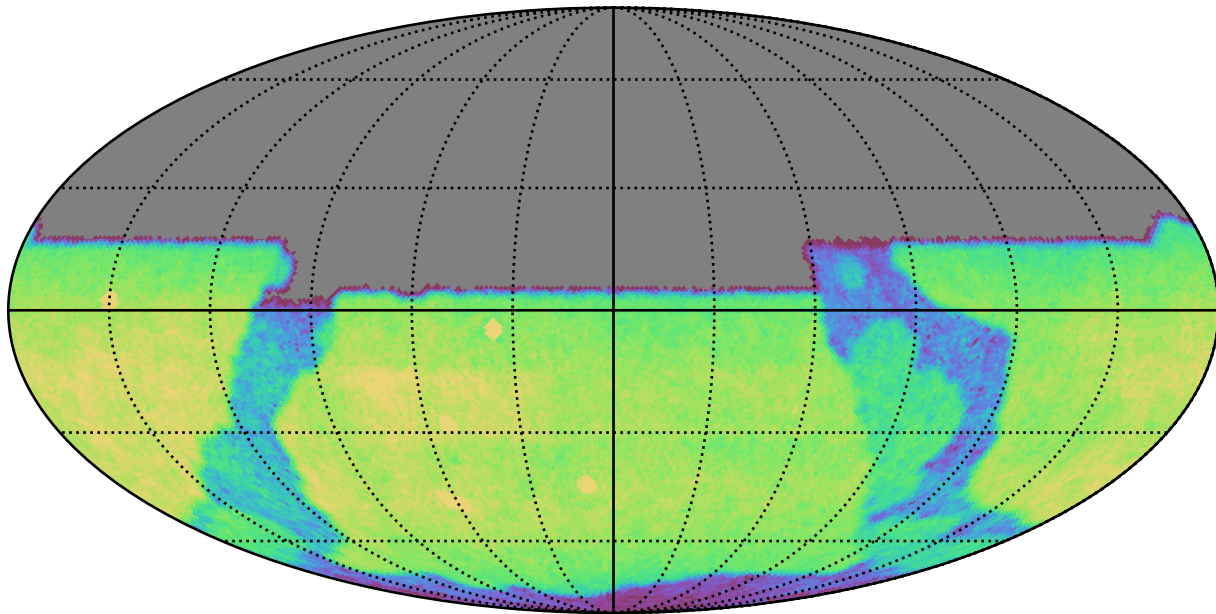
reweight_plane_v3.3_10yrs All sky u band: CoaddM5
