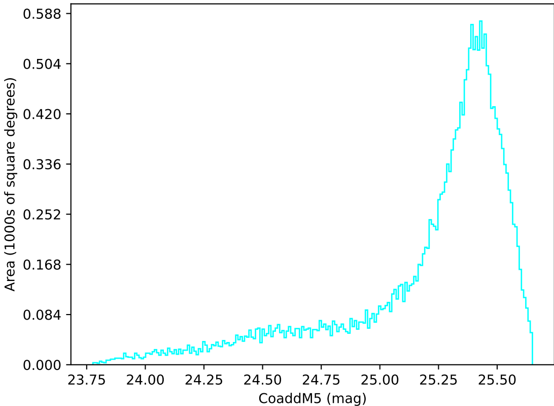
reweight_plane_v3.3_10yrs All sky u band: CoaddM5
