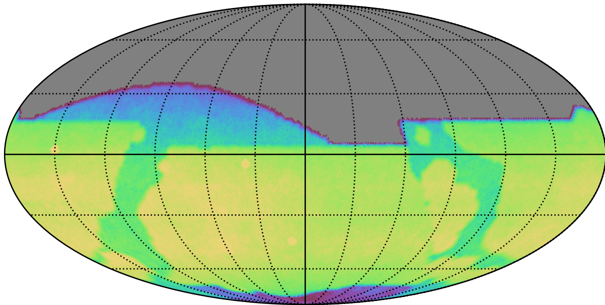
reweight_plane_v3.3_10yrs All sky r band: CoaddM5
