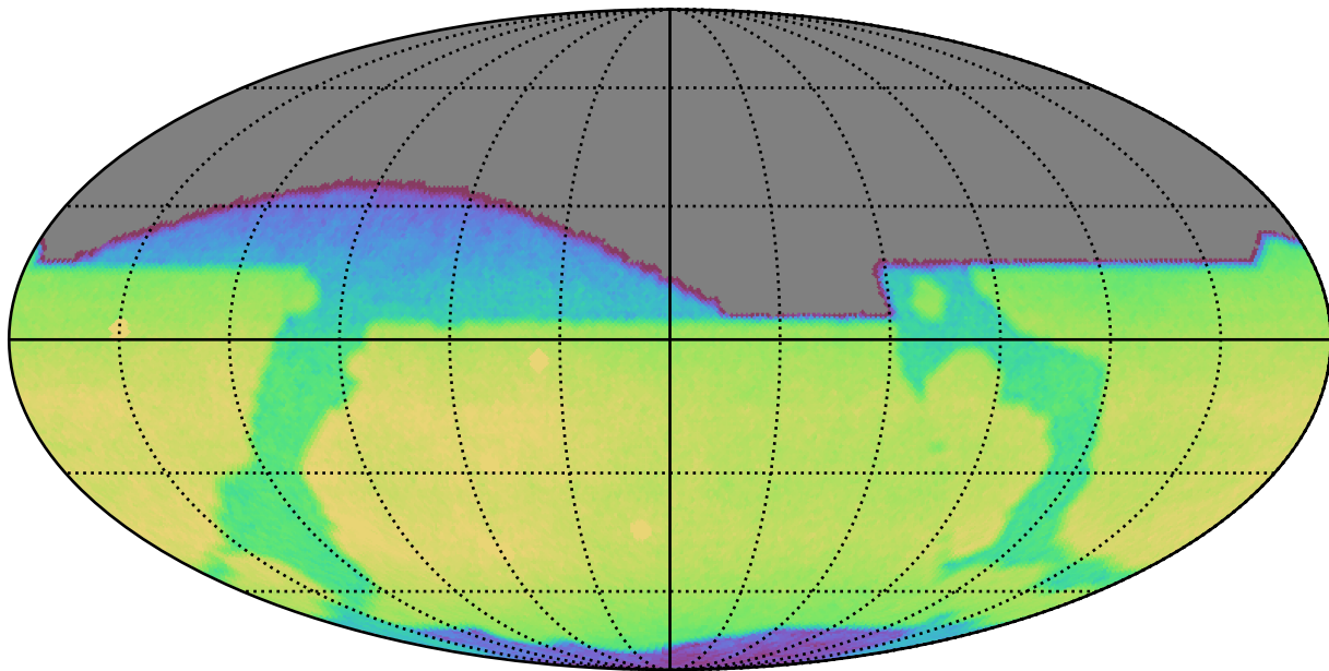
reweight_plane_v3.3_10yrs All sky i band: CoaddM5
