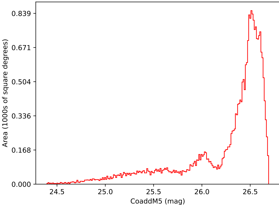
reweight_plane_v3.3_10yrs All sky i band: CoaddM5
