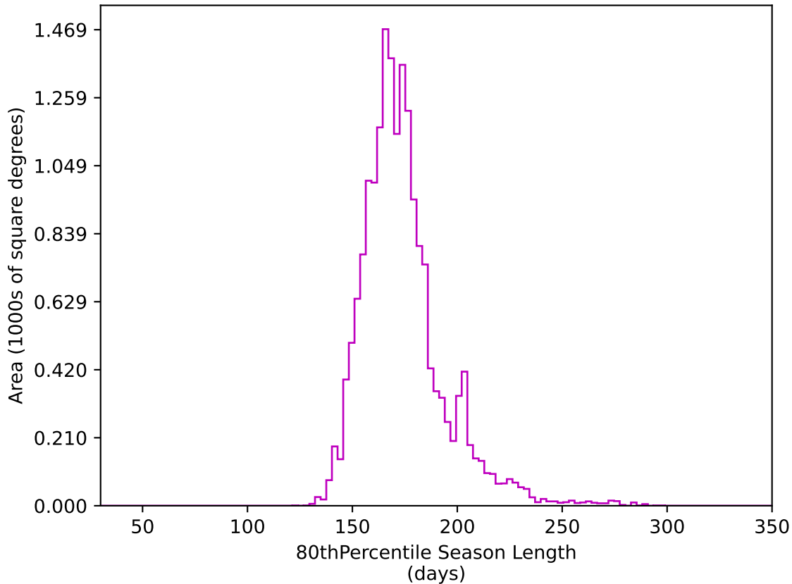
reweight_plane_v3.3_10yrs WFD z band: 80thPercentile Season Length
