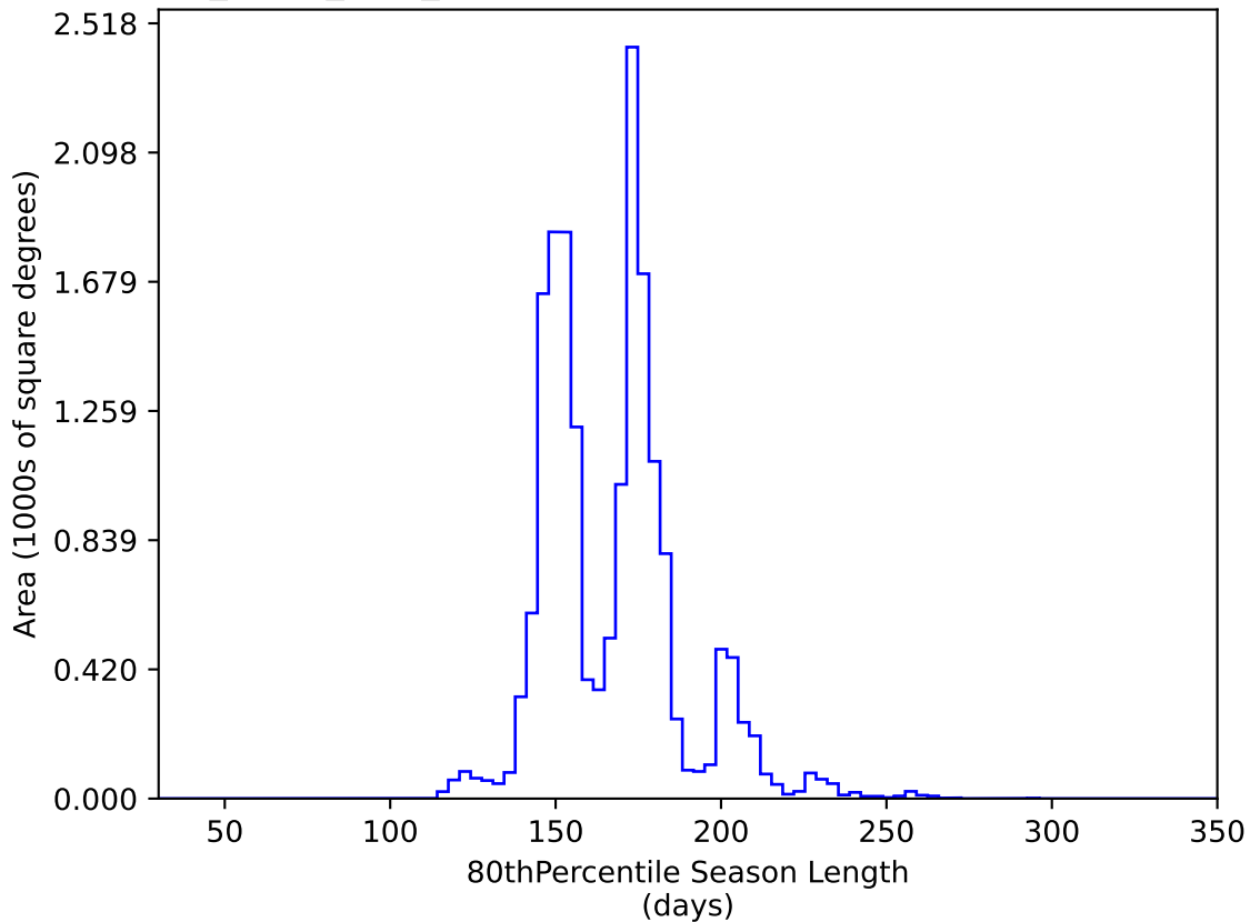
reweight_plane_v3.3_10yrs WFD y band: 80thPercentile Season Length
