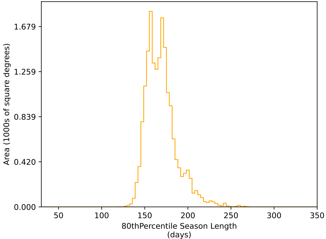
reweight_plane_v3.3_10yrs WFD r band: 80thPercentile Season Length
