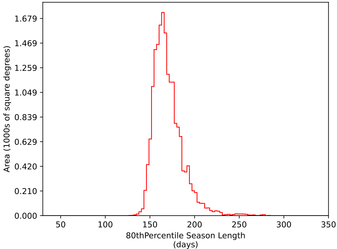
reweight_plane_v3.3_10yrs WFD i band: 80thPercentile Season Length
