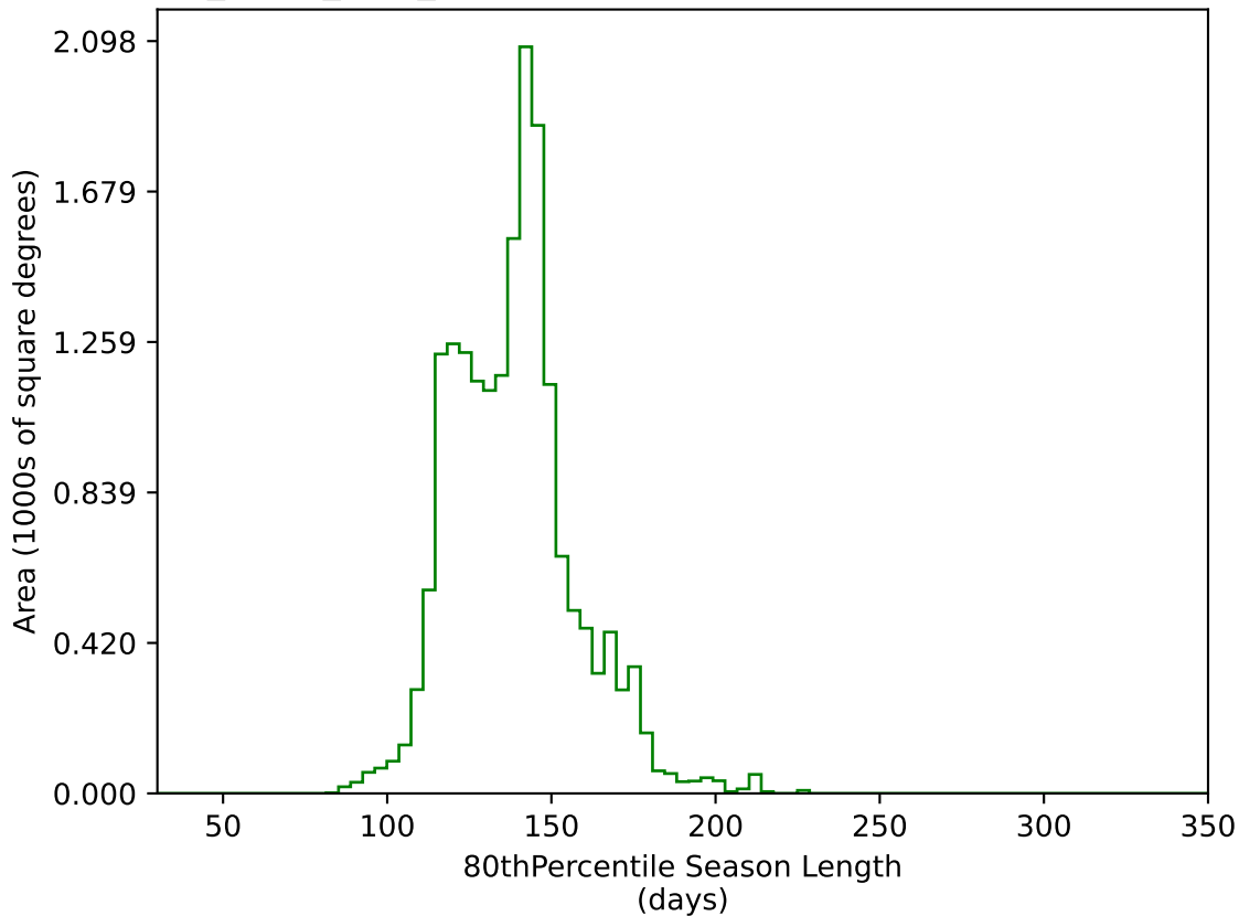
reweight_plane_v3.3_10yrs WFD g band: 80thPercentile Season Length
