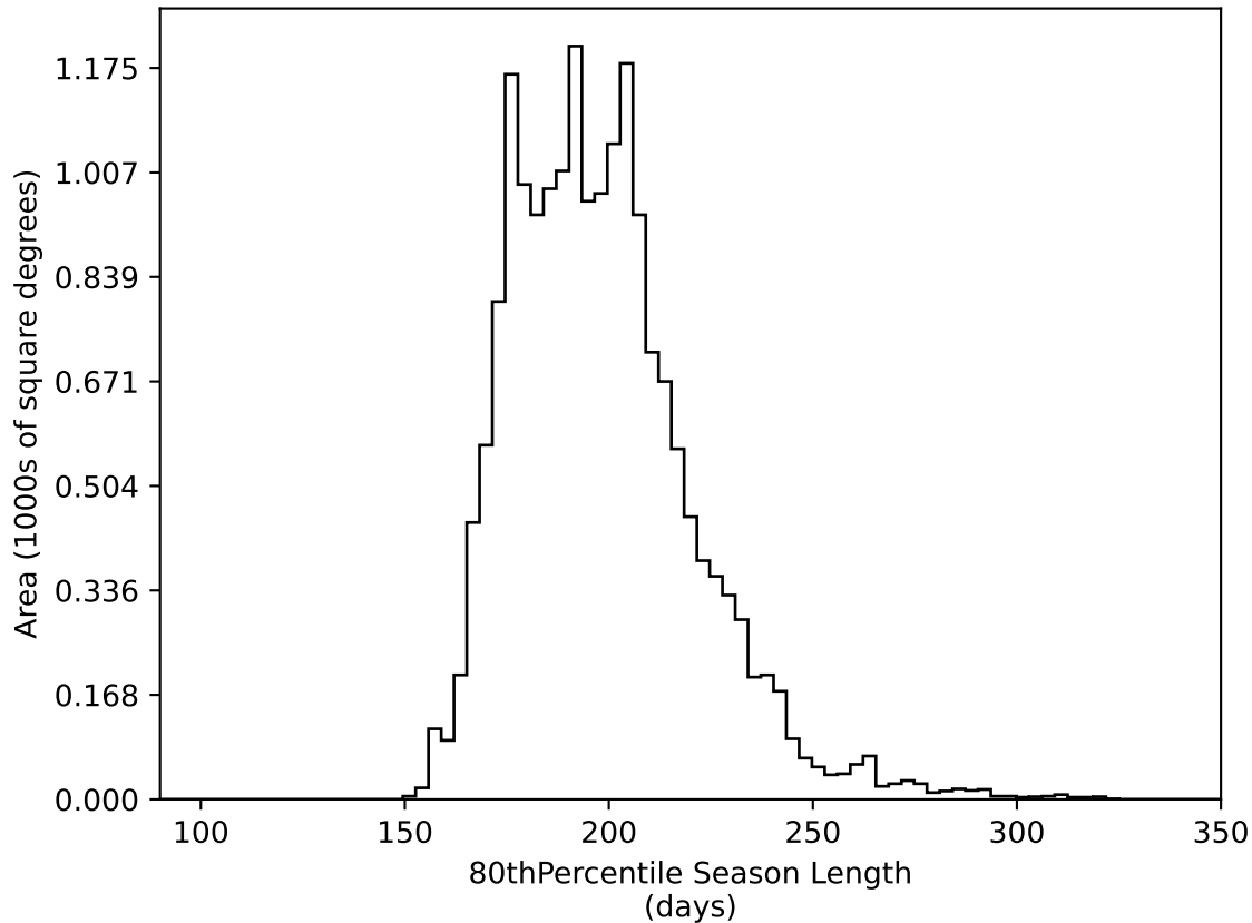
reweight_plane_v3.3_10yrs WFD all bands: 80thPercentile Season Length
