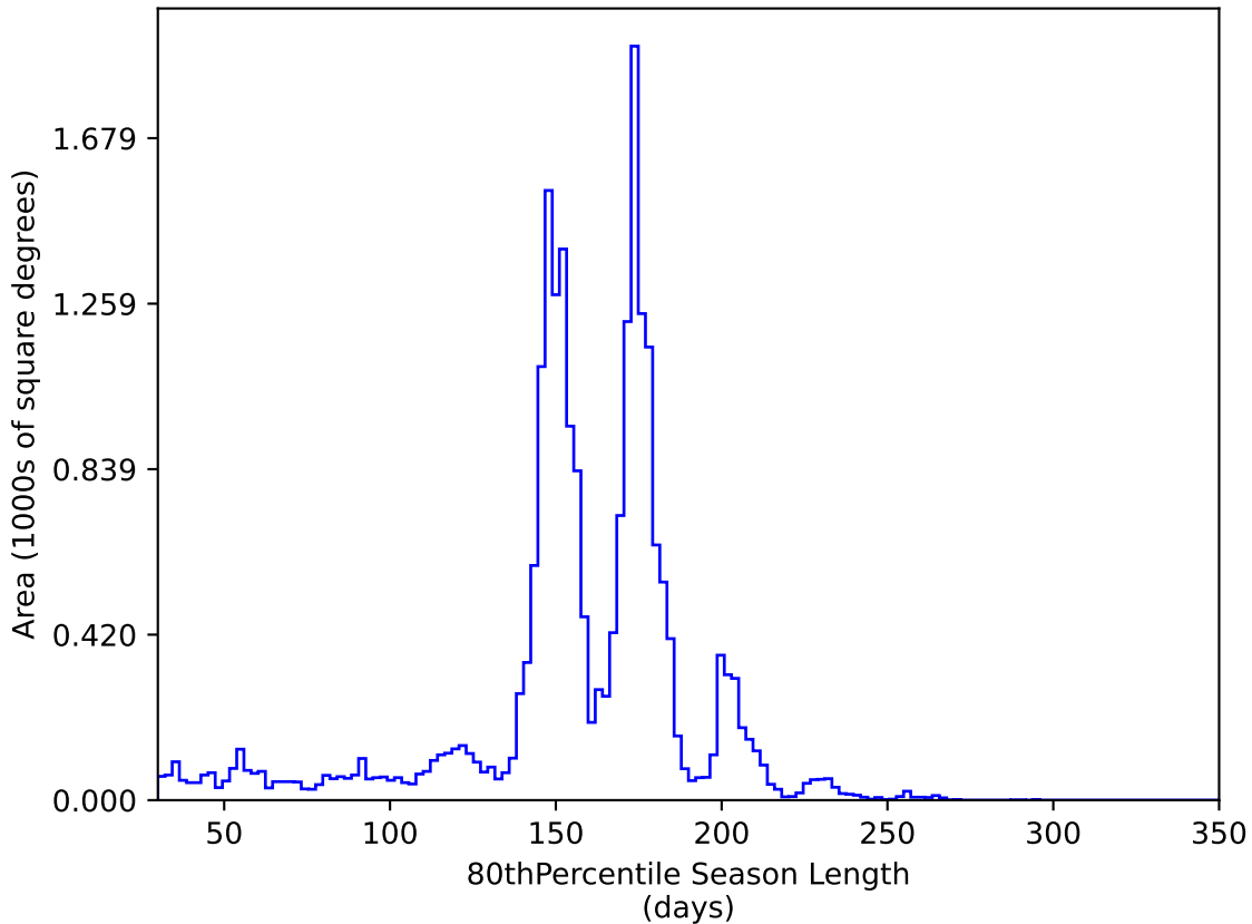
reweight_plane_v3.3_10yrs All sky y band: 80thPercentile Season Length
