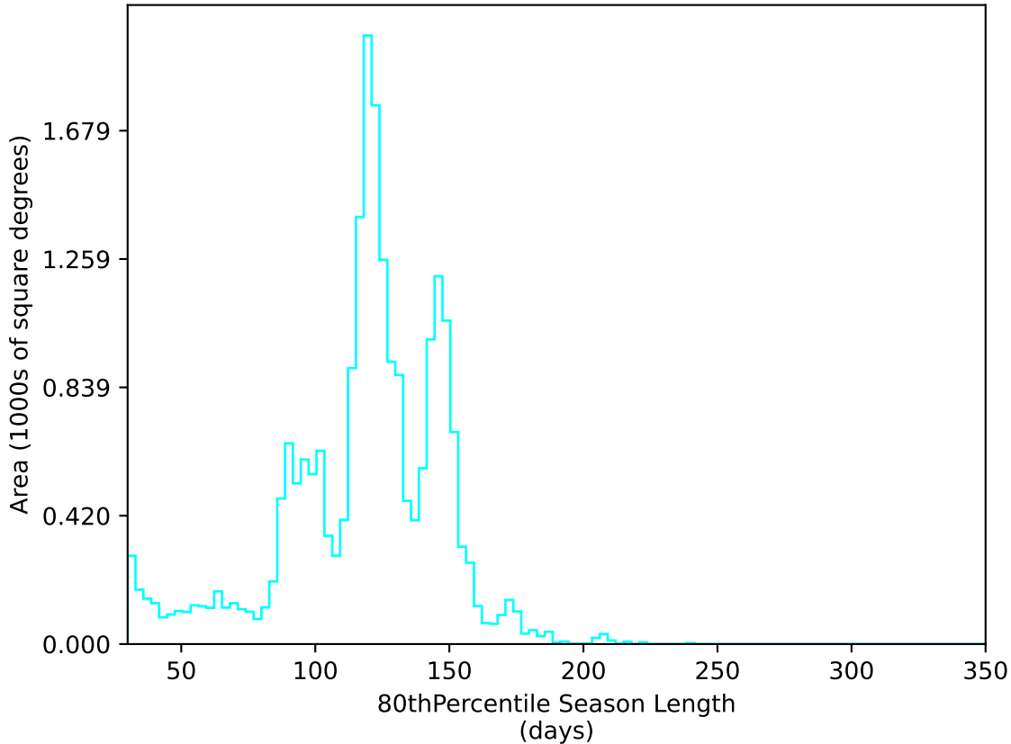
reweight_plane_v3.3_10yrs All sky u band: 80thPercentile Season Length
