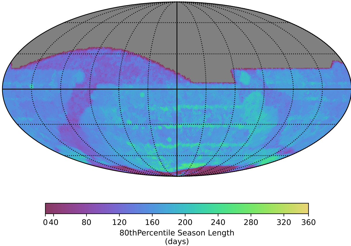
reweight_plane_v3.3_10yrs All sky r band: 80thPercentile Season Length
