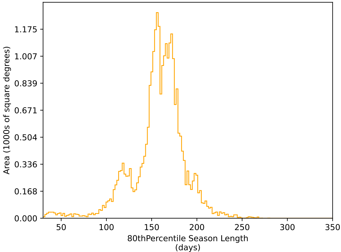
reweight_plane_v3.3_10yrs All sky r band: 80thPercentile Season Length
