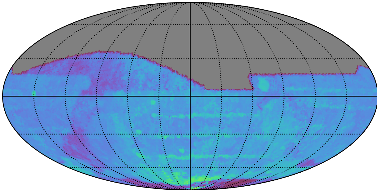
reweight_plane_v3.3_10yrs All sky i band: 80thPercentile Season Length
