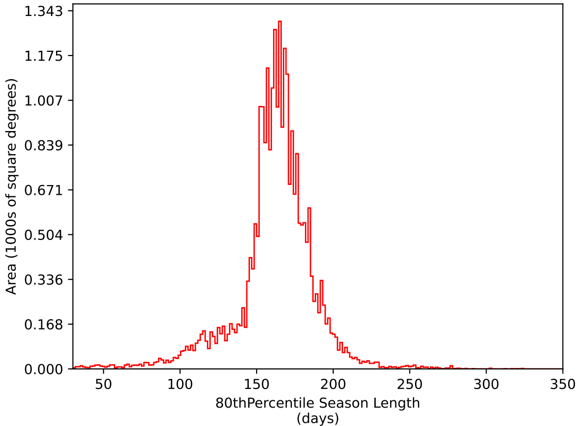
reweight_plane_v3.3_10yrs All sky i band: 80thPercentile Season Length
