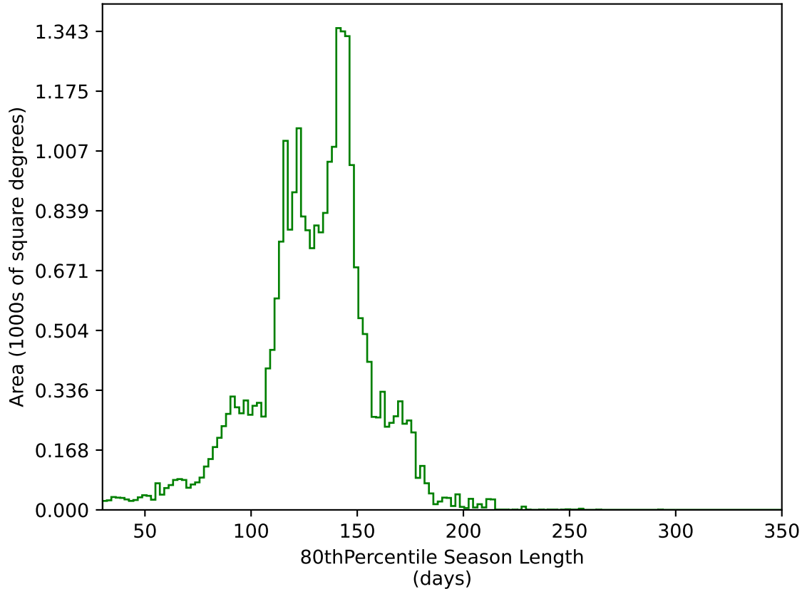
reweight_plane_v3.3_10yrs All sky g band: 80thPercentile Season Length
