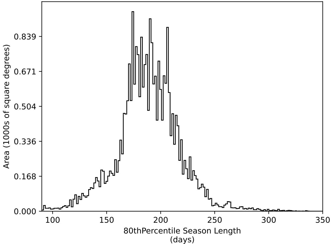
reweight_plane_v3.3_10yrs All sky all bands: 80thPercentile Season Length
