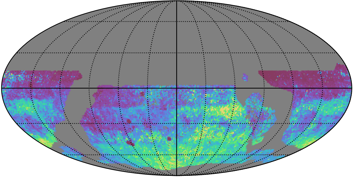
reweight_plane_v3.3_10yrs WFD zy bands: 75th Percentile Intranight Timespan
